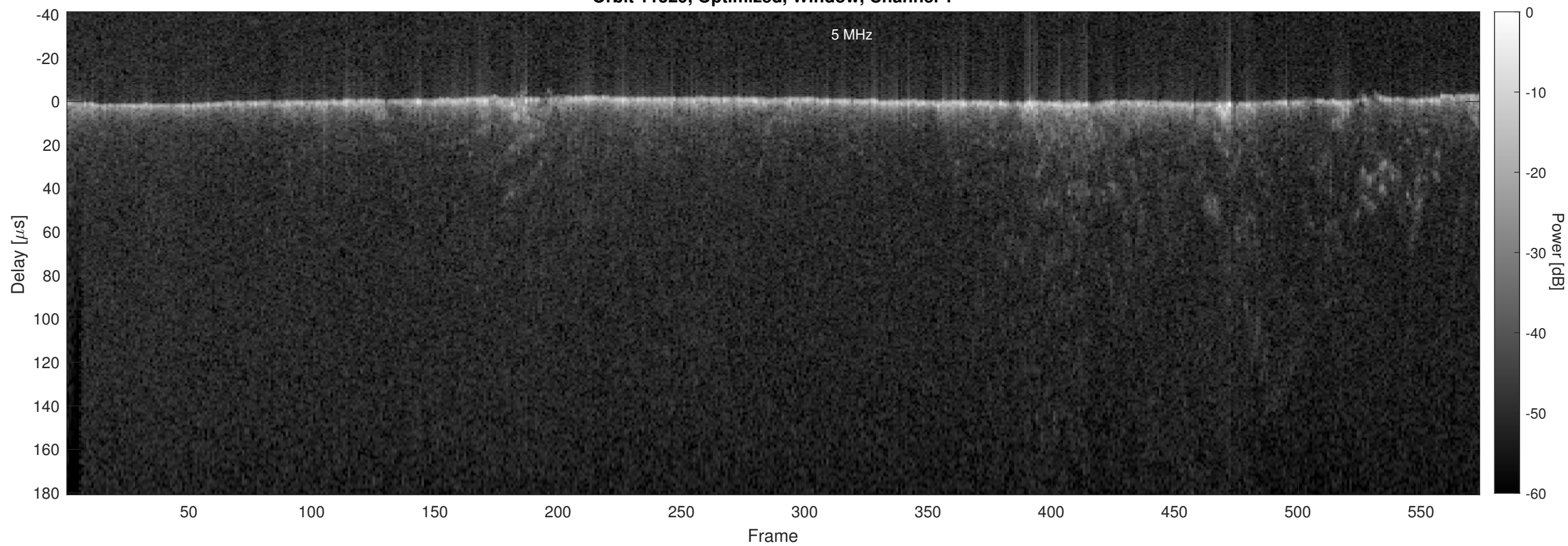
Orbit 11529, Optimized, Window, Channel 2
