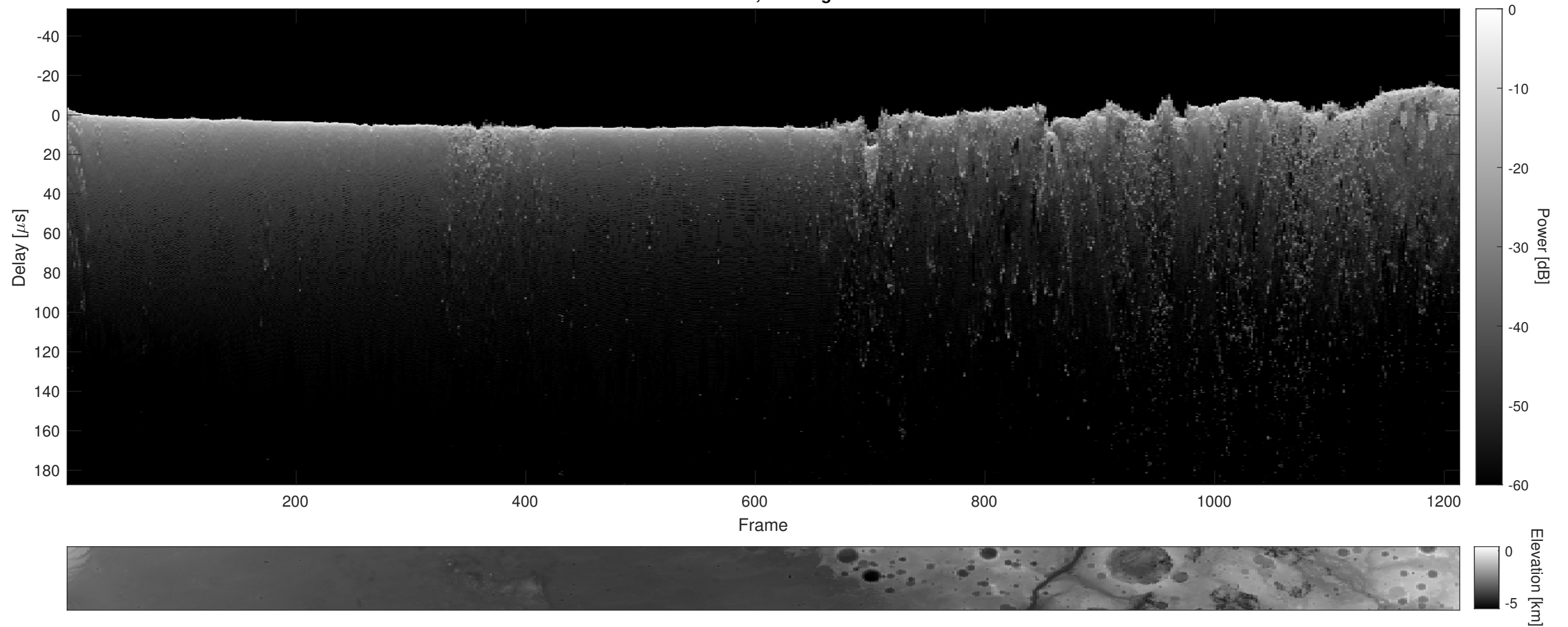
Orbit 11530, Cluttergram
