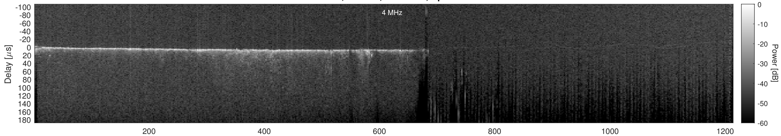
Orbit 11530, Cluttergram
