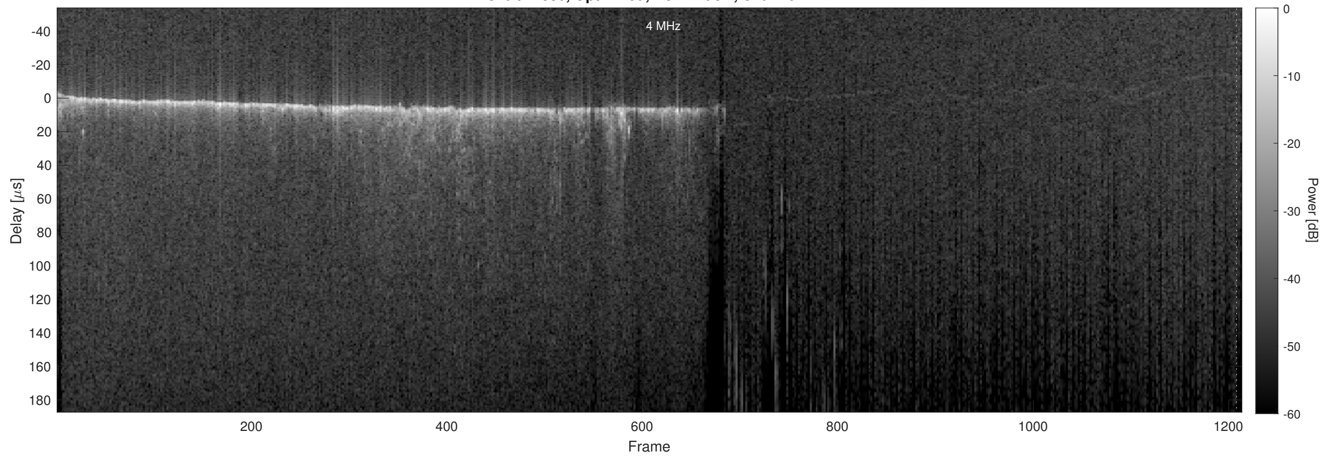
Orbit 11530, Optimized, No Window, Channel 2
