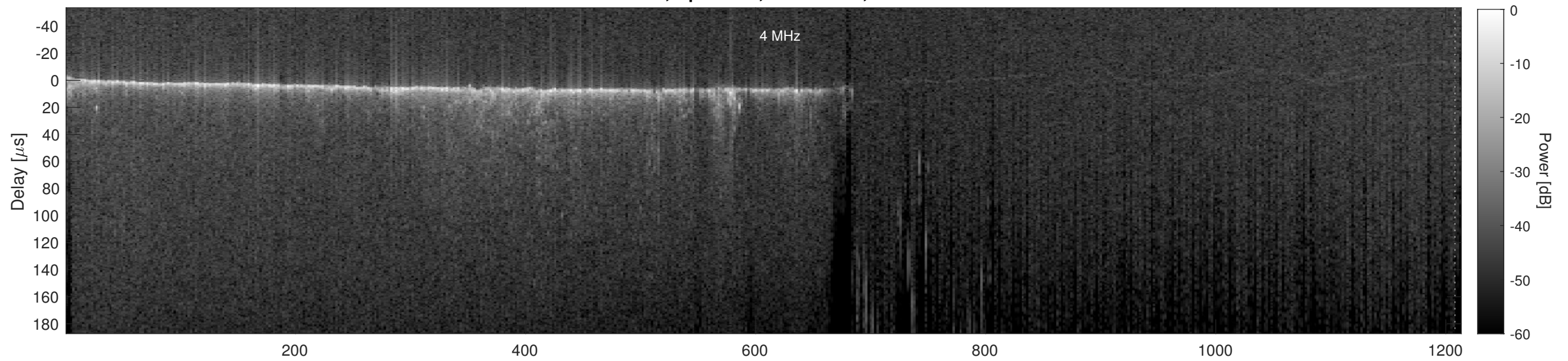
Orbit 11530, Cluttergram
