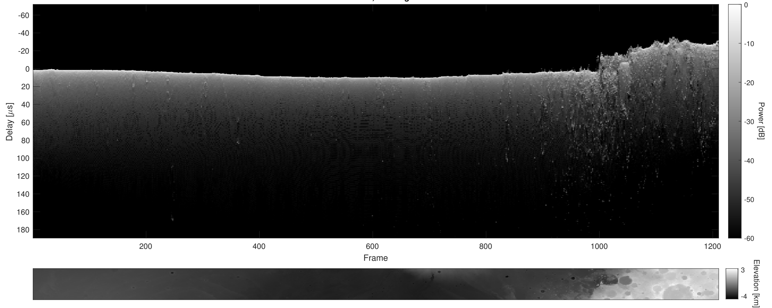
Orbit 11532, Cluttergram
