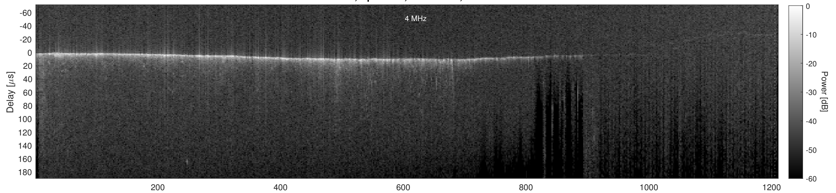
Orbit 11532, Cluttergram
