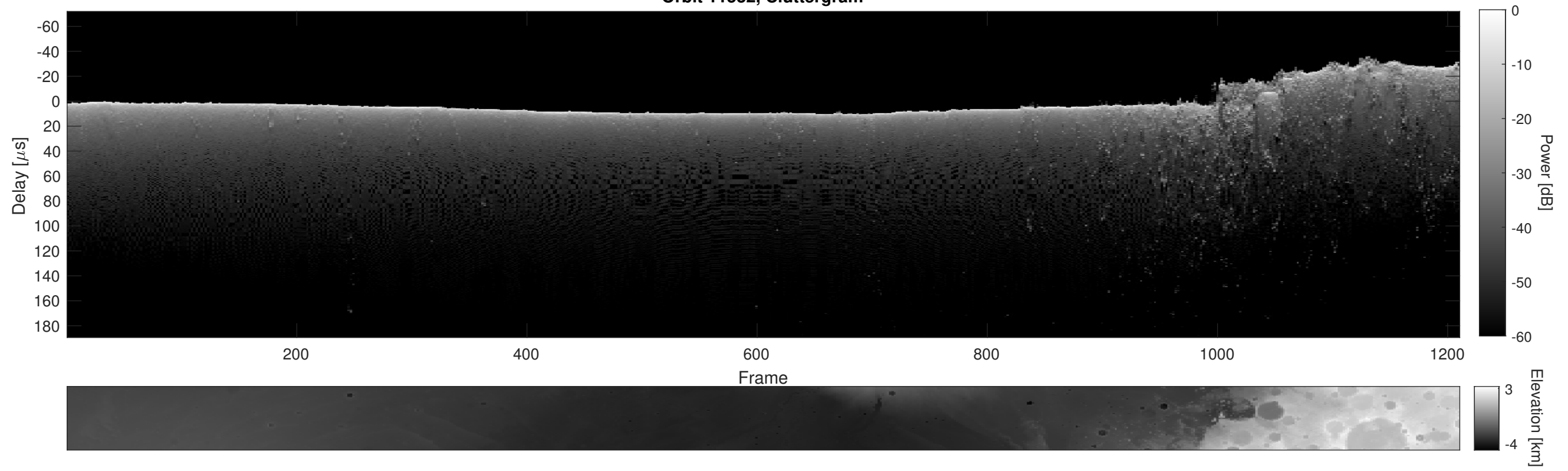
Orbit 11532, Cluttergram
