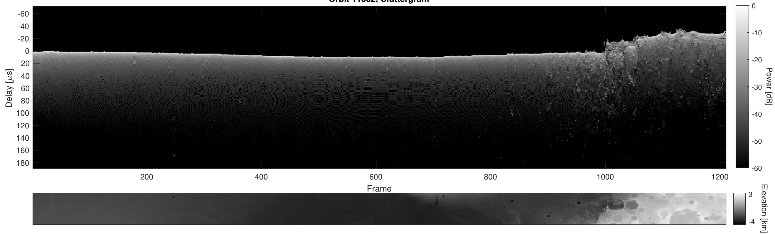
Orbit 11532, Cluttergram
