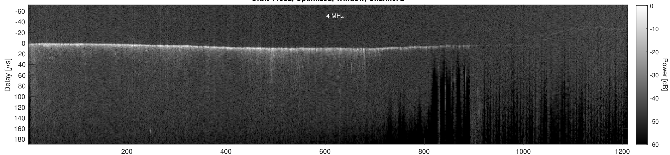
Orbit 11532, Cluttergram
