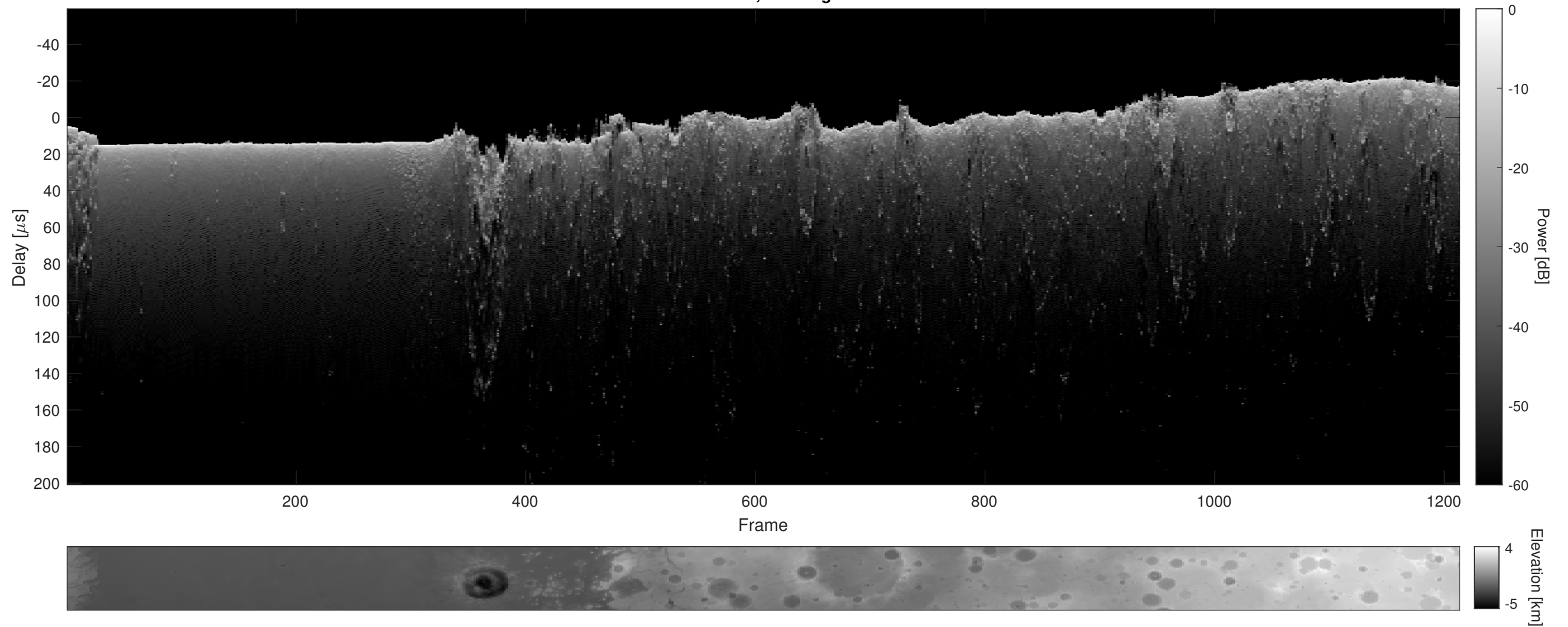
Orbit 11533, Cluttergram
