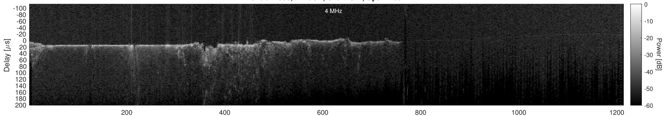
Orbit 11533, Cluttergram
