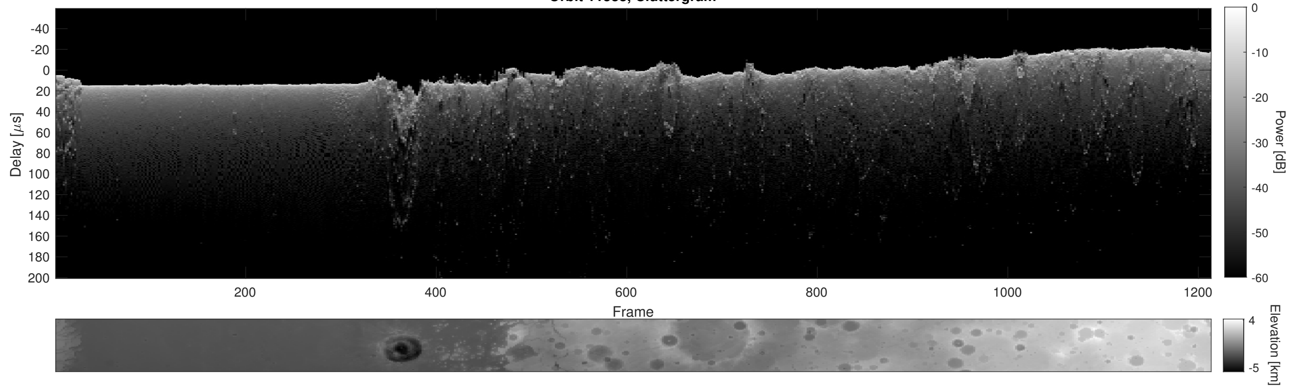
Orbit 11533, Cluttergram
