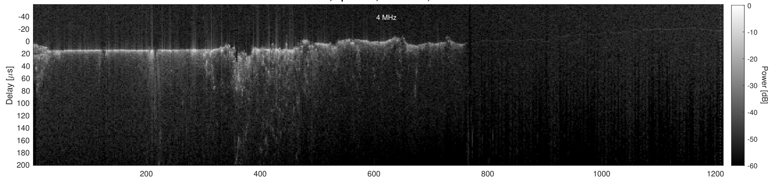
Orbit 11533, Cluttergram
