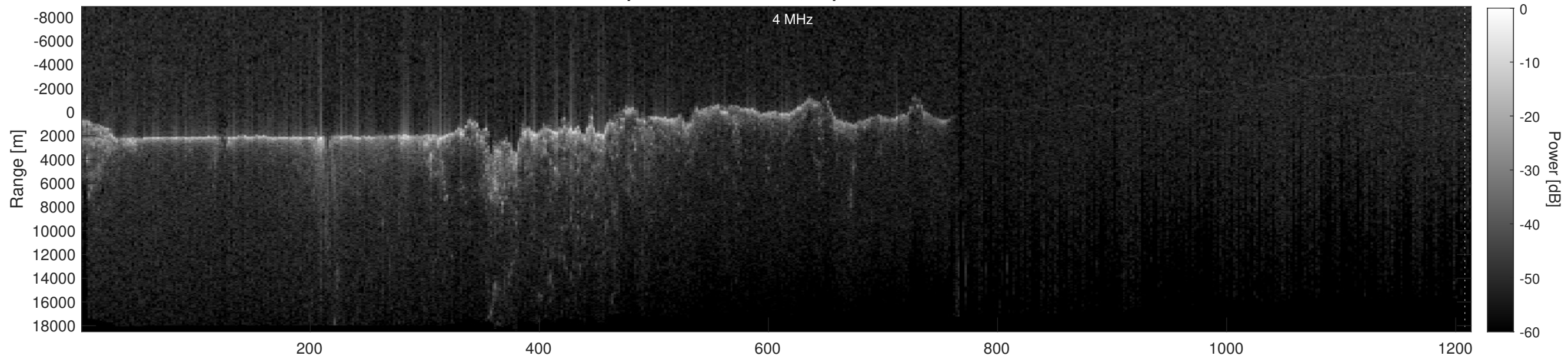
Orbit 11533, Depth-Corrected Cluttergram
