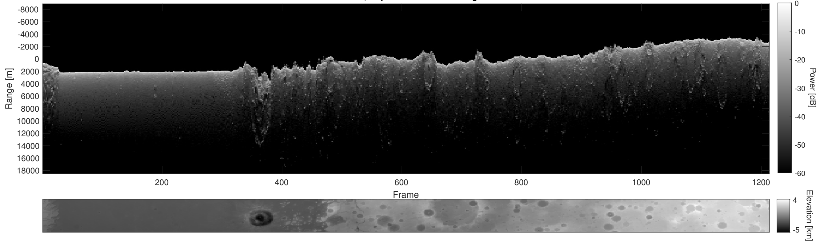
Orbit 11533, Depth-Corrected Cluttergram
