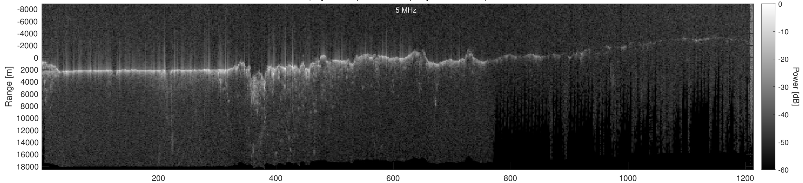
Orbit 11533, Optimized, No Window, Depth-Corrected, Channel 2
