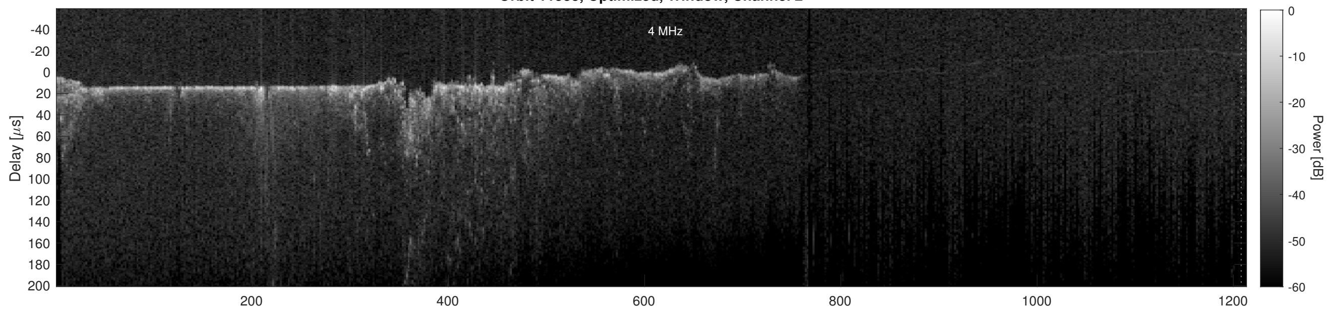
Orbit 11533, Cluttergram
