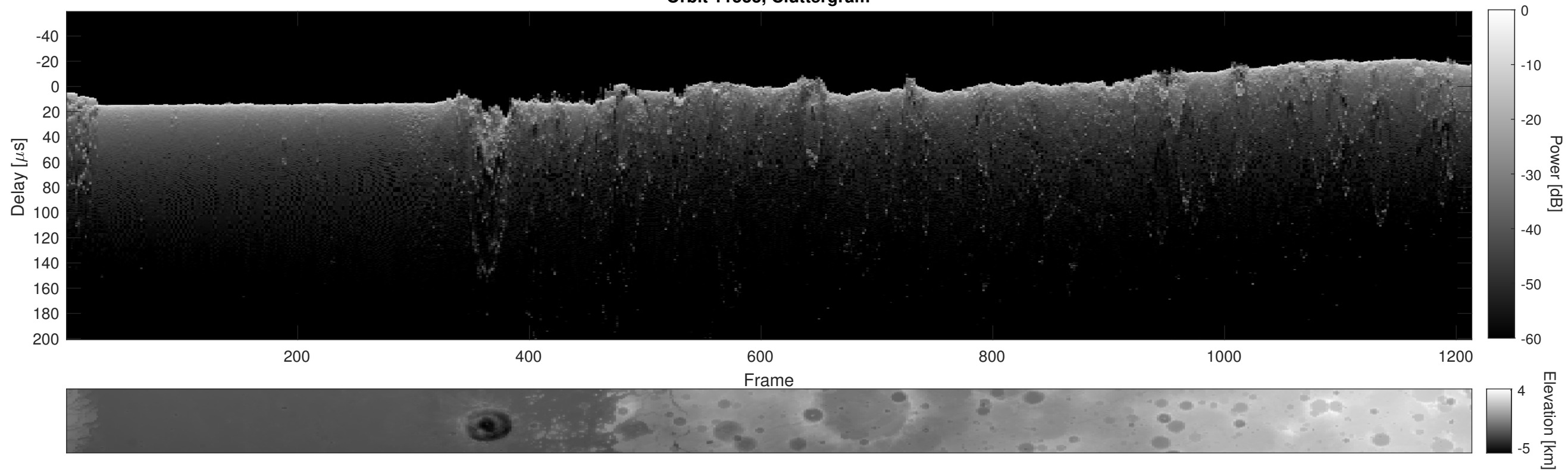
Orbit 11533, Cluttergram
