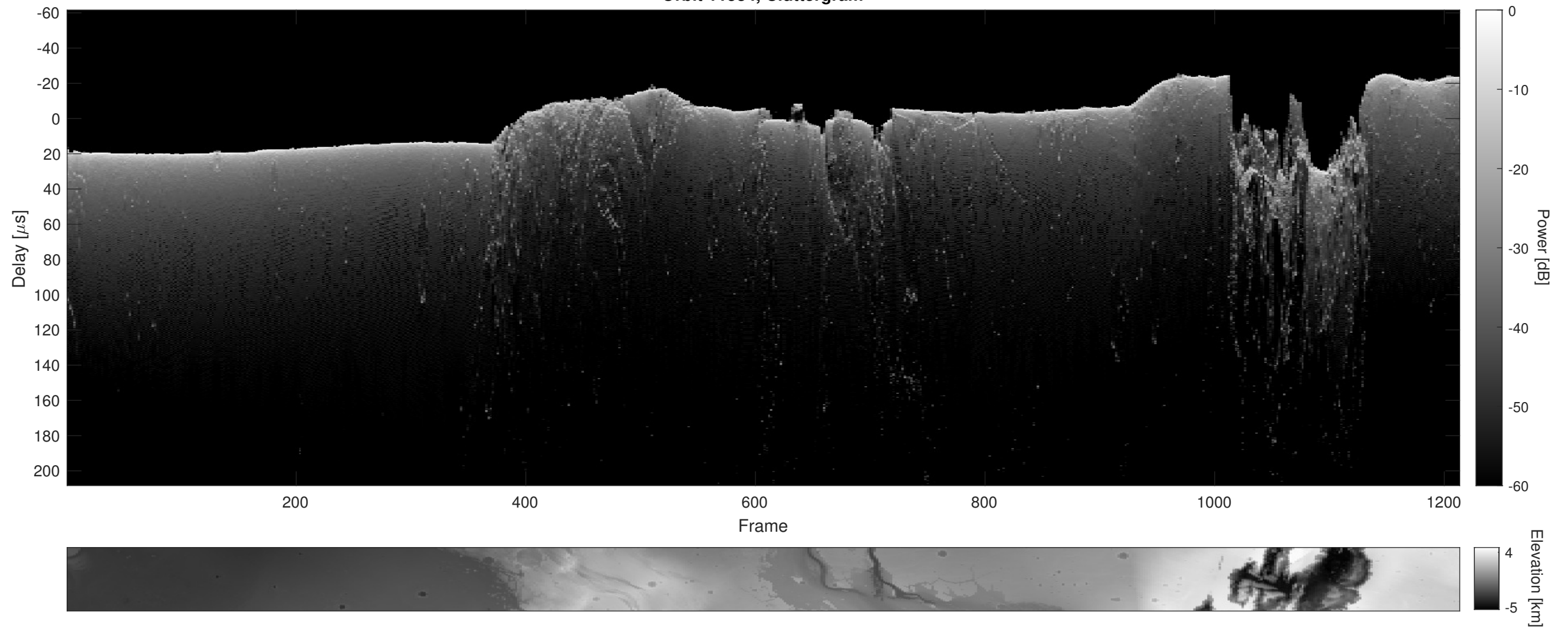
Orbit 11534, Cluttergram
