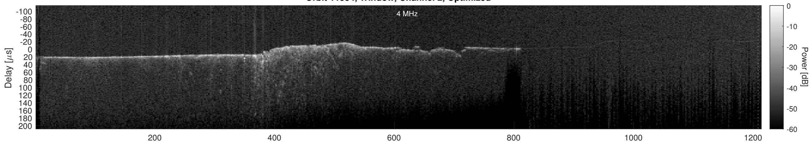
Orbit 11534, Cluttergram
