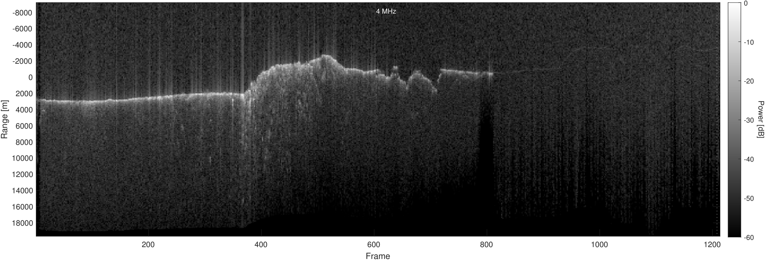
Orbit 11534, Optimized, No Window, Depth-Corrected, Channel 2
