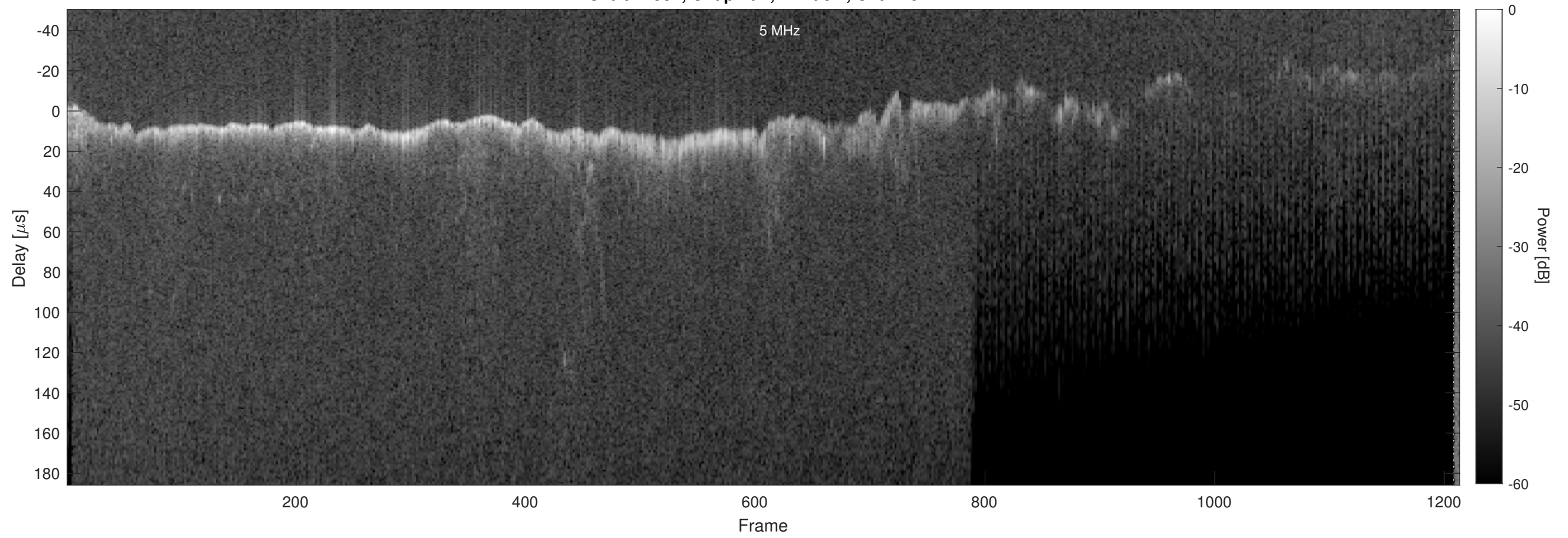
Orbit 11537, Chapman, Window, Channel 2
