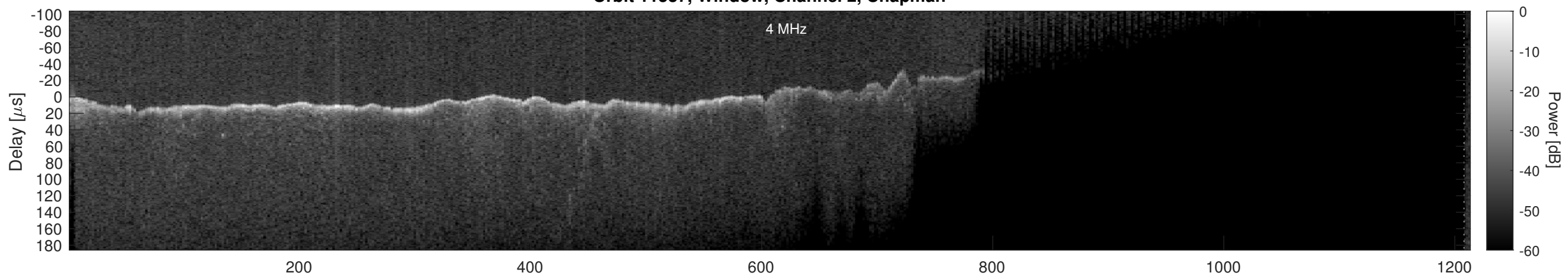
Orbit 11537, Window, Channel 2, Optimized
