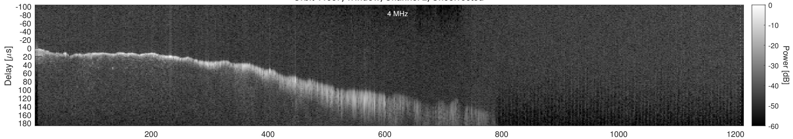
Orbit 11537, Window, Channel 2, Chapman
