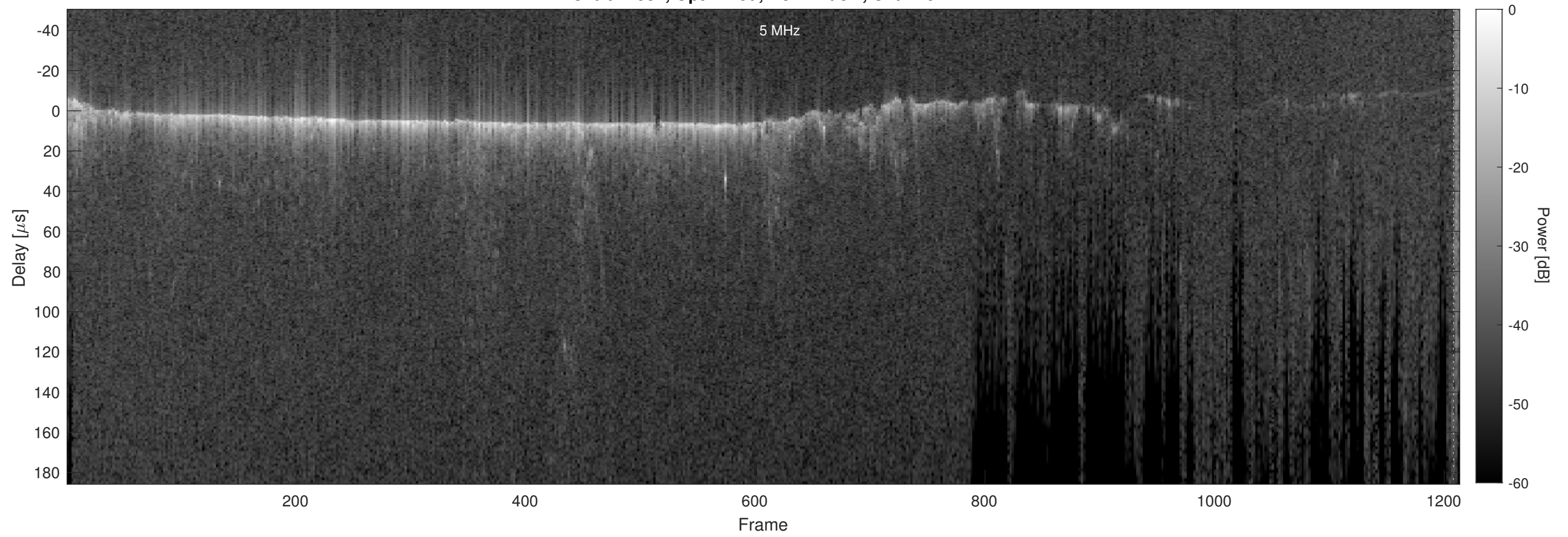
Orbit 11537, Optimized, No Window, Channel 2
