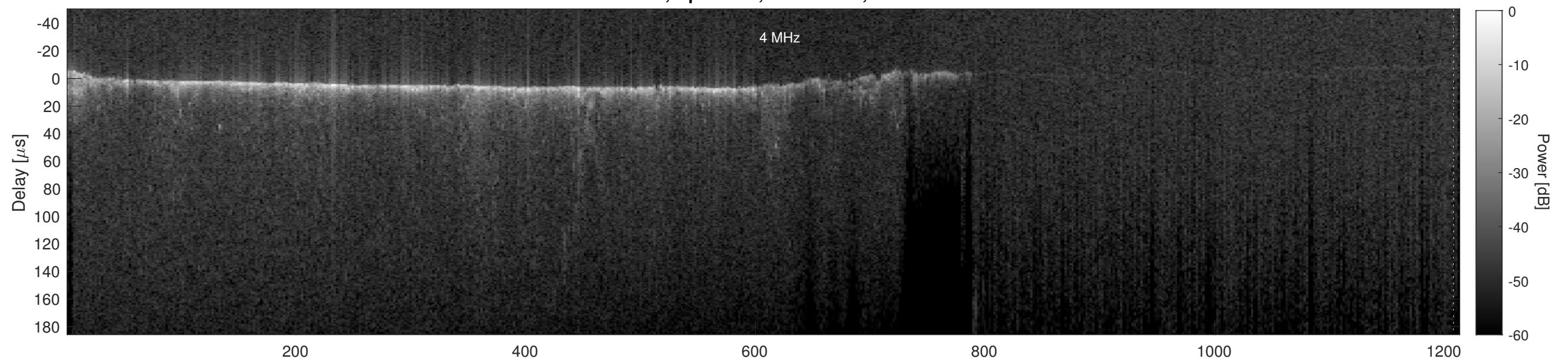
Orbit 11537, Cluttergram
