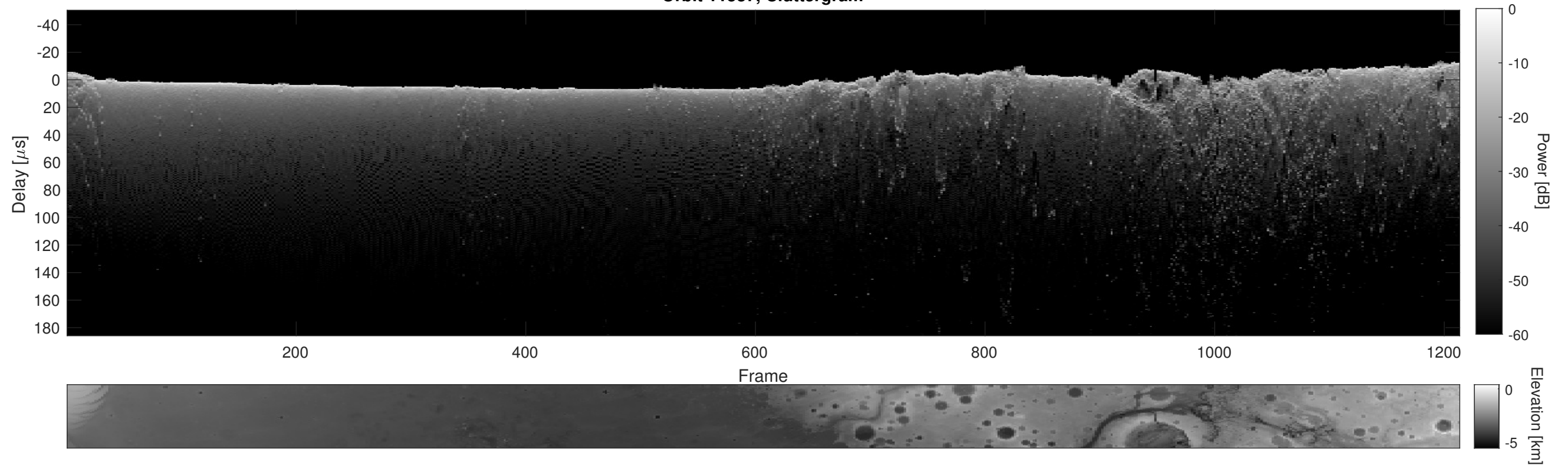
Orbit 11537, Cluttergram
