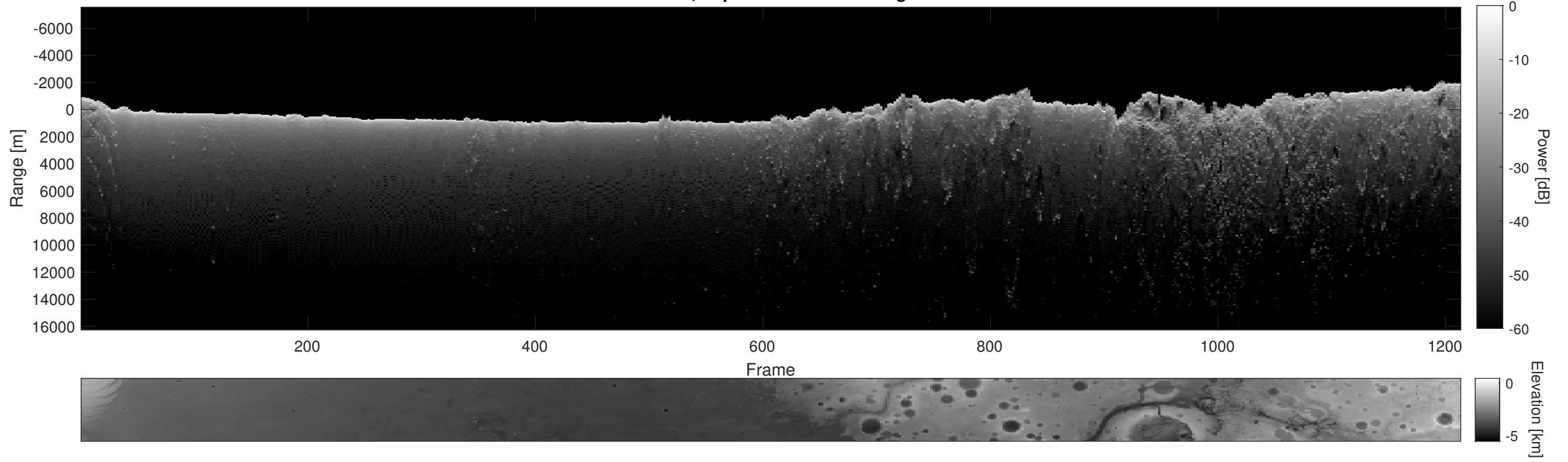
Orbit 11537, Depth-Corrected Cluttergram
