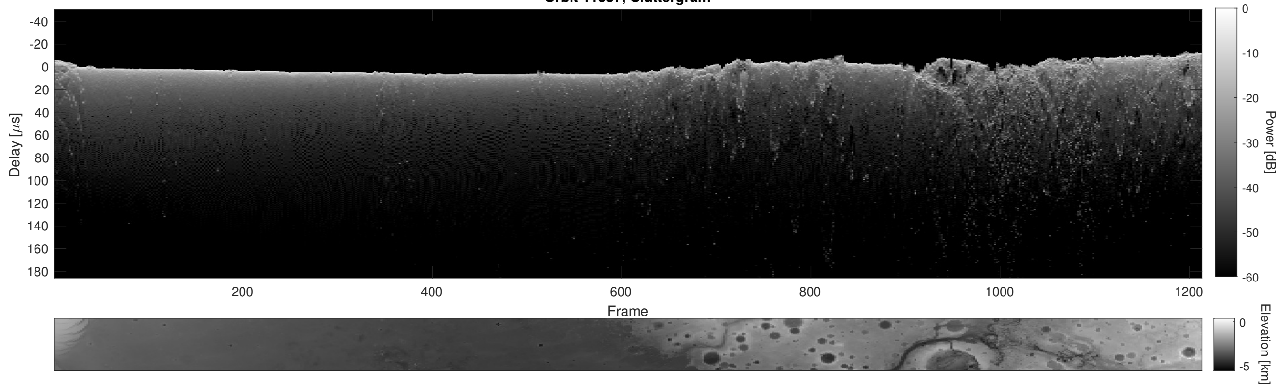
Orbit 11537, Cluttergram
