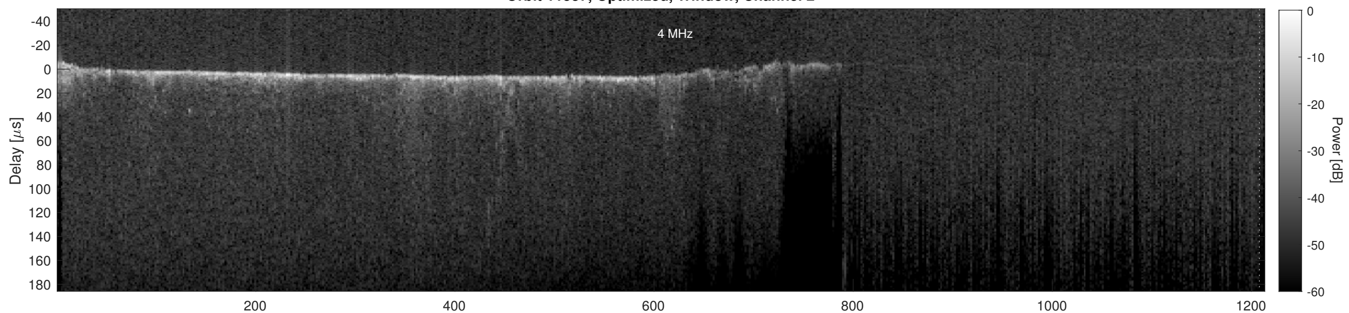
Orbit 11537, Cluttergram
