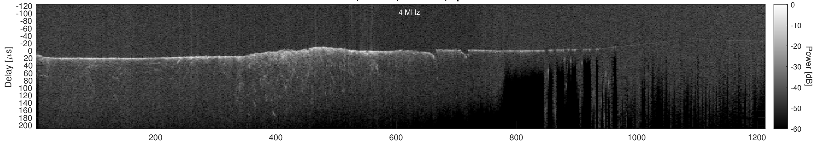
Orbit 11541, Cluttergram
