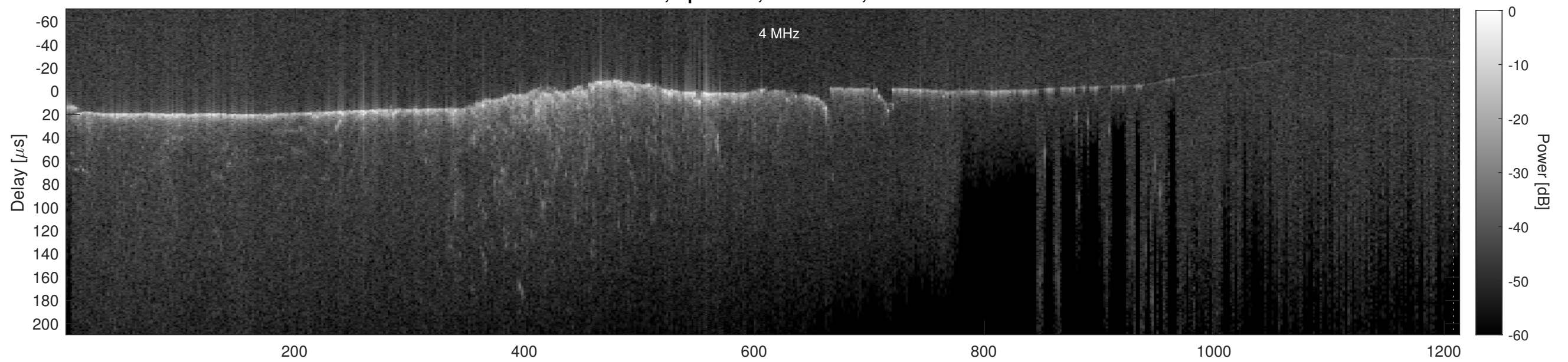
Orbit 11541, Cluttergram
