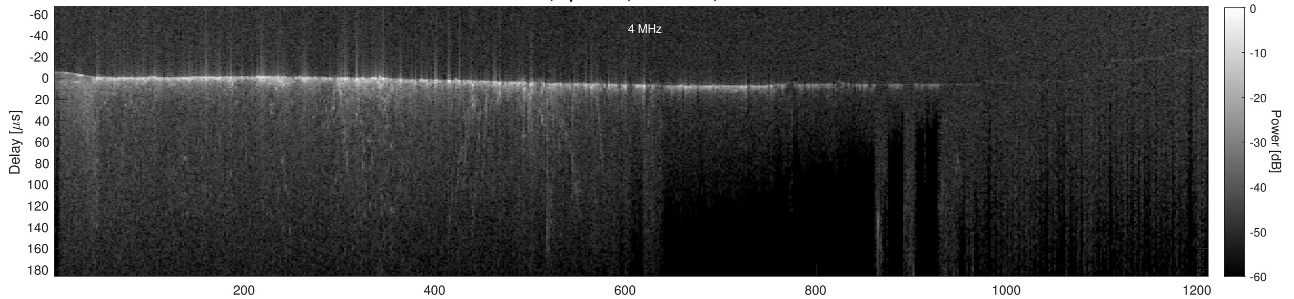
Orbit 11542, Cluttergram
