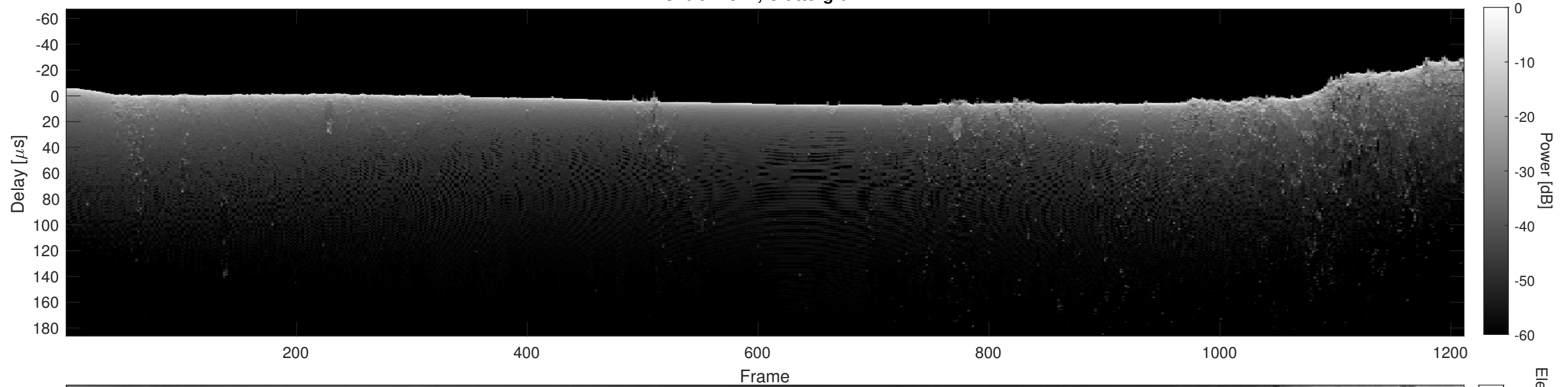
Orbit 11542, Cluttergram
