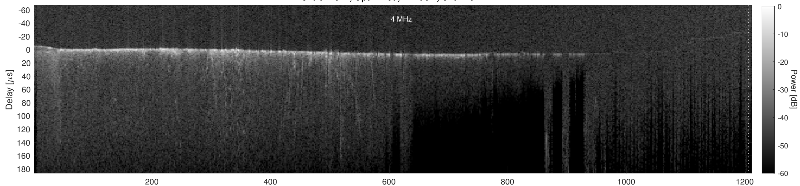
Orbit 11542, Cluttergram
