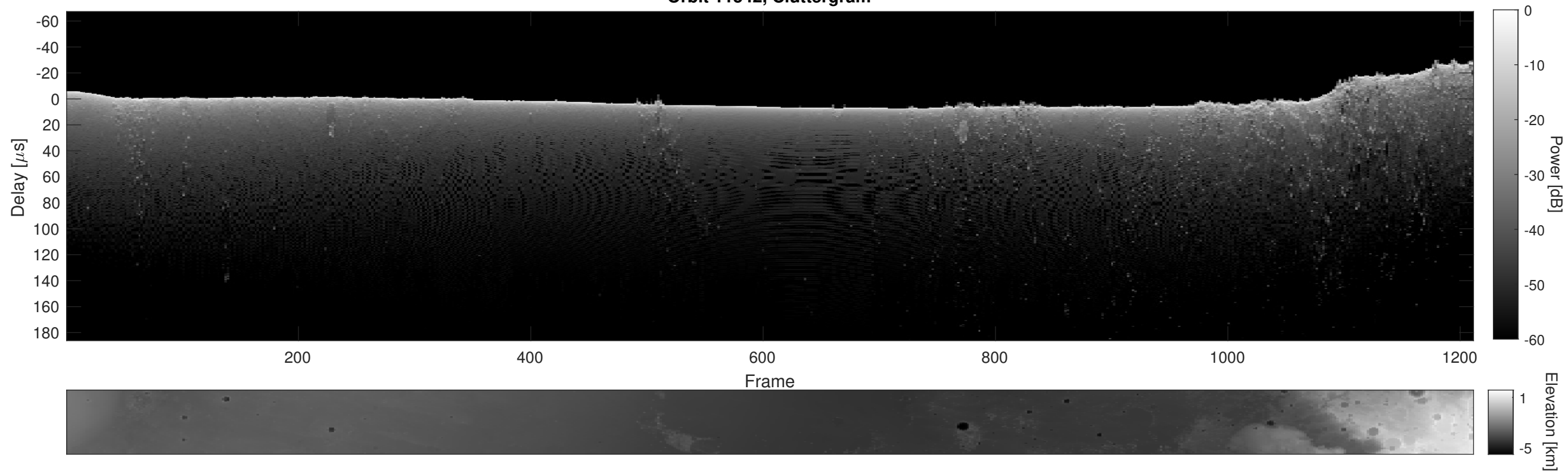
Orbit 11542, Cluttergram
