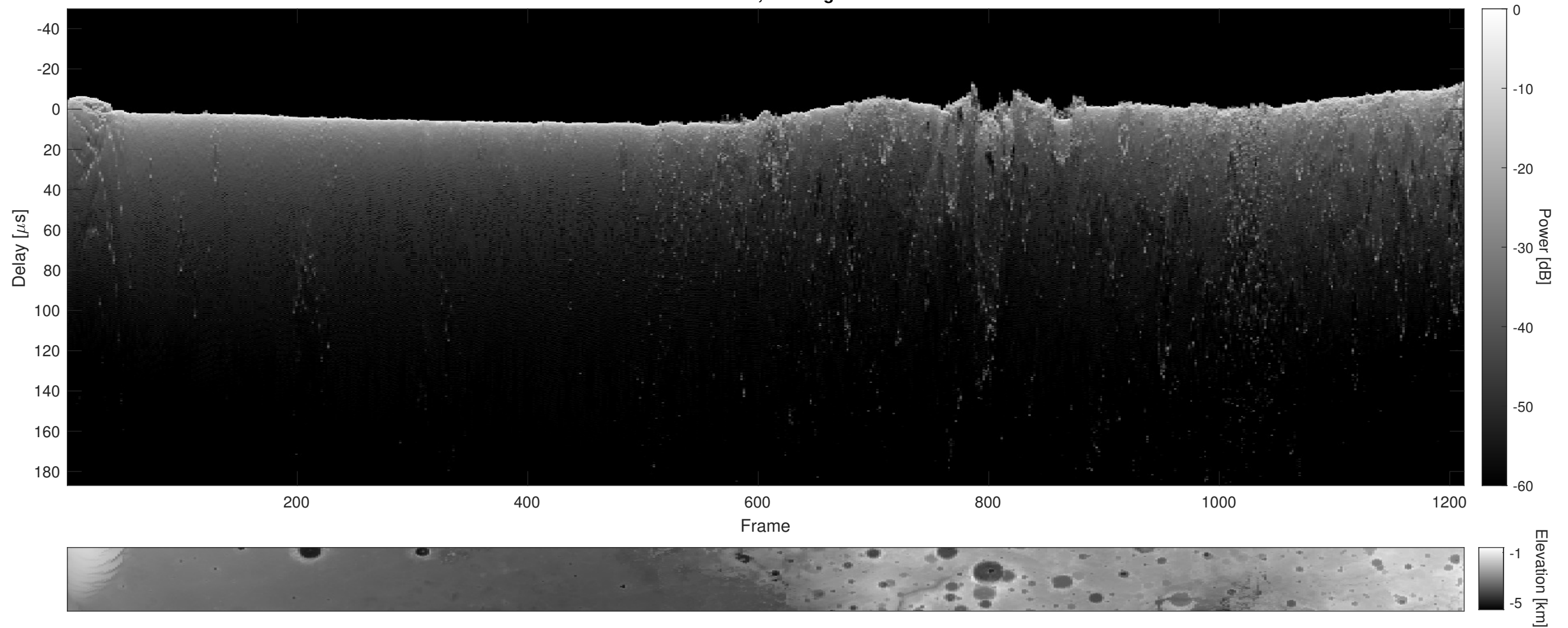
Orbit 11544, Cluttergram
