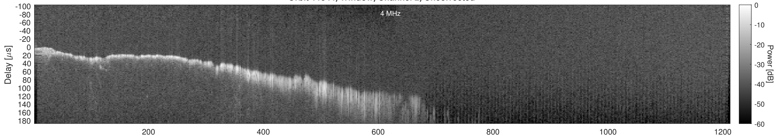
Orbit 11544, Window, Channel 2, Chapman
