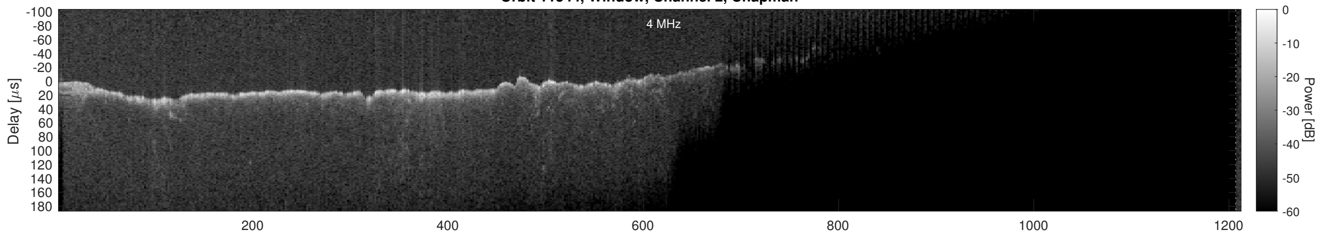
Orbit 11544, Window, Channel 2, Optimized
