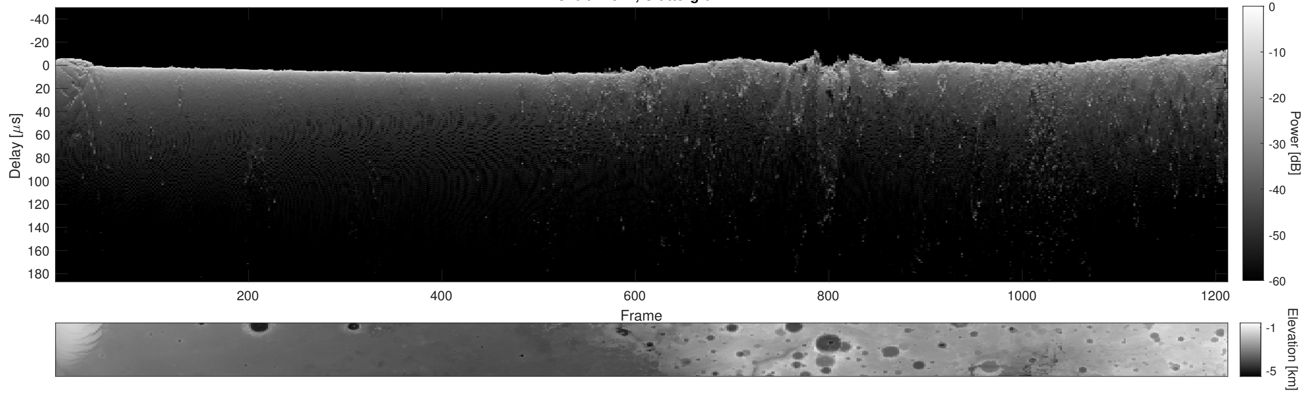
Orbit 11544, Cluttergram
