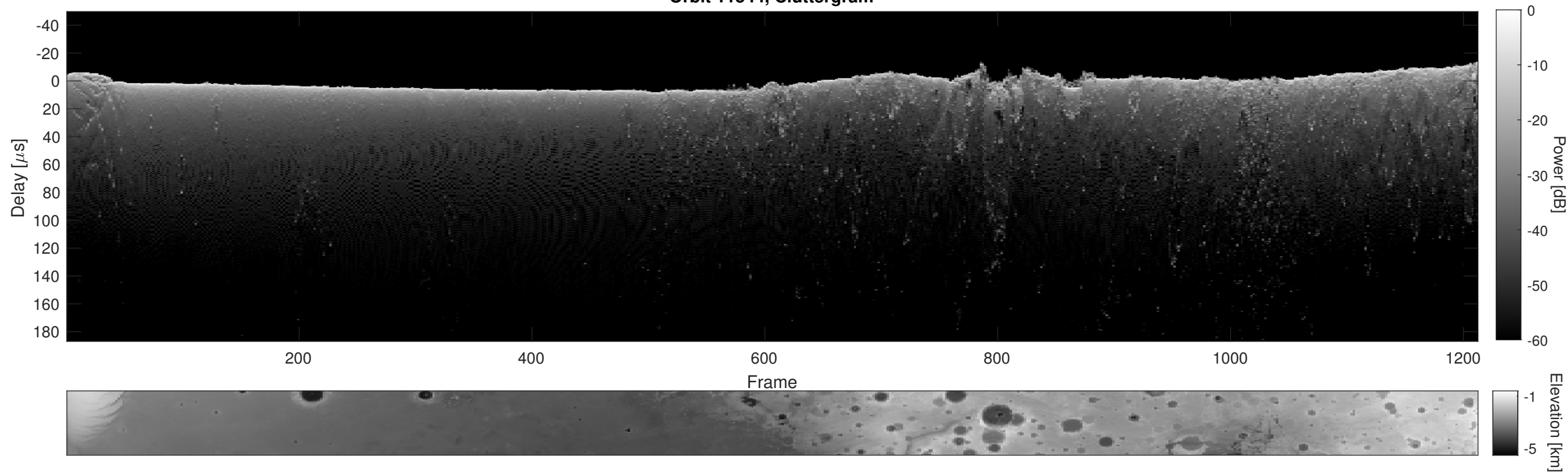
Orbit 11544, Cluttergram
