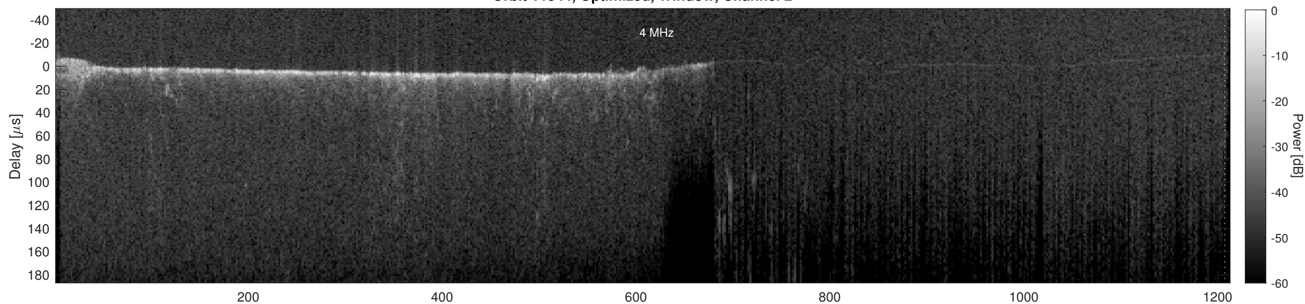
Orbit 11544, Cluttergram
