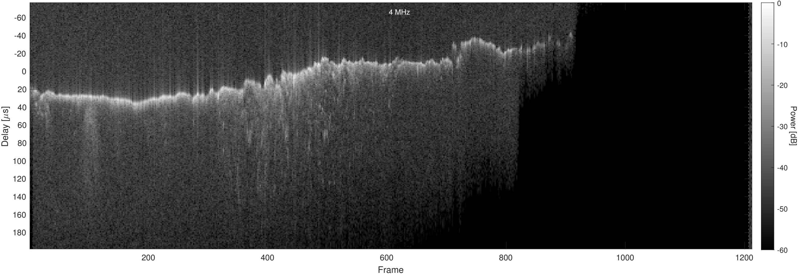
Orbit 11548, Chapman, No Window, Channel 2
