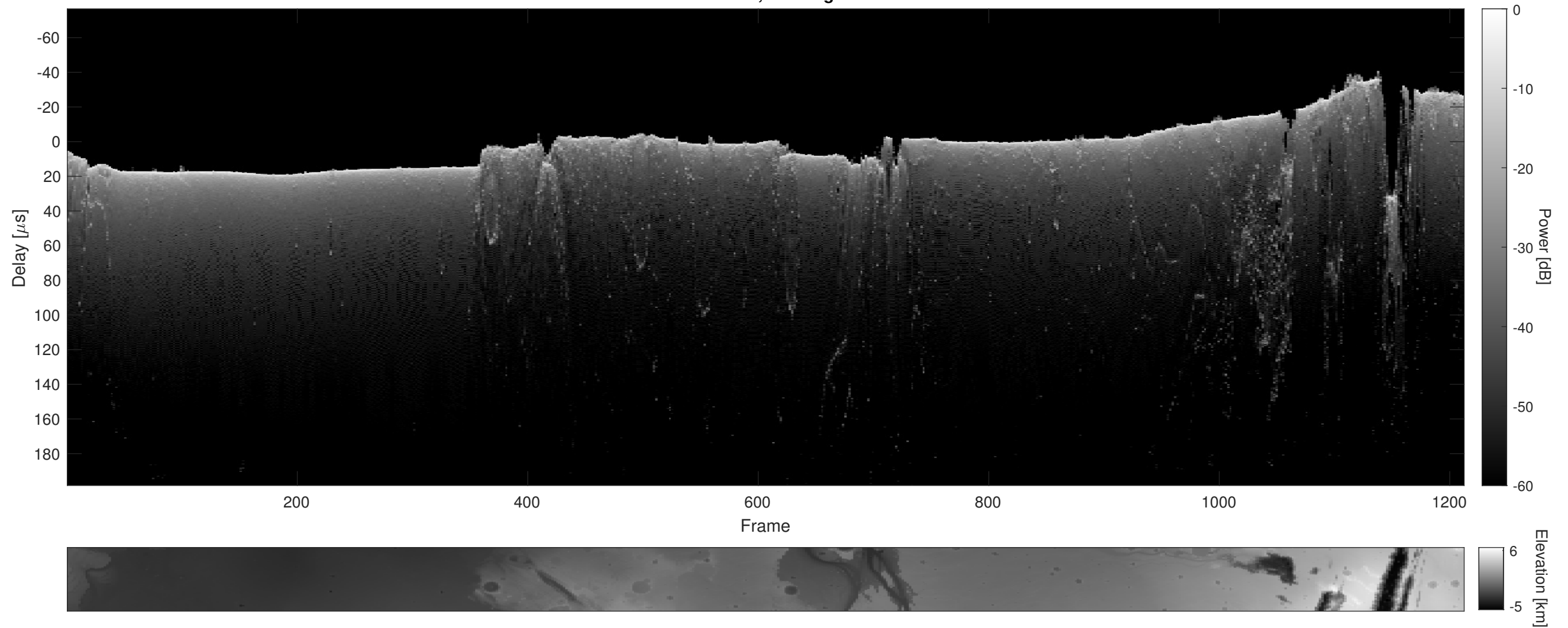
Orbit 11548, Cluttergram
