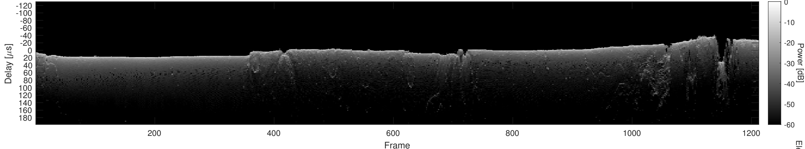
Orbit 11548, Cluttergram
