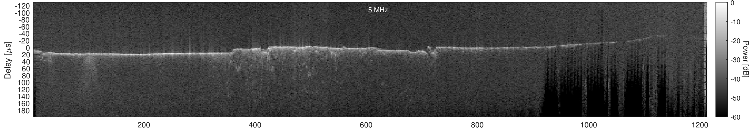
Orbit 11548, Cluttergram
