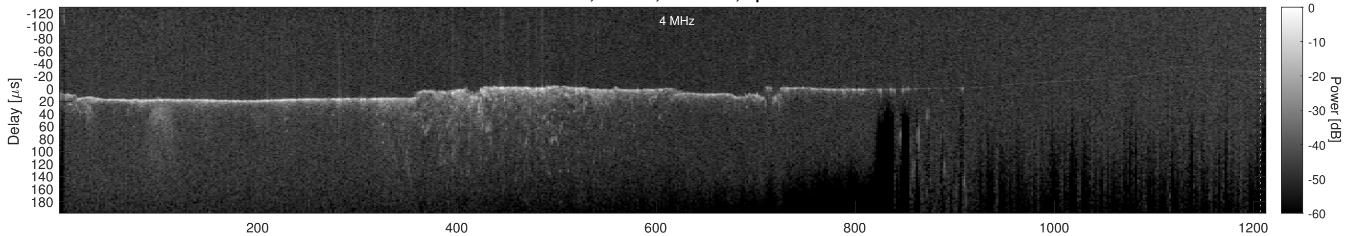
Orbit 11548, Cluttergram
