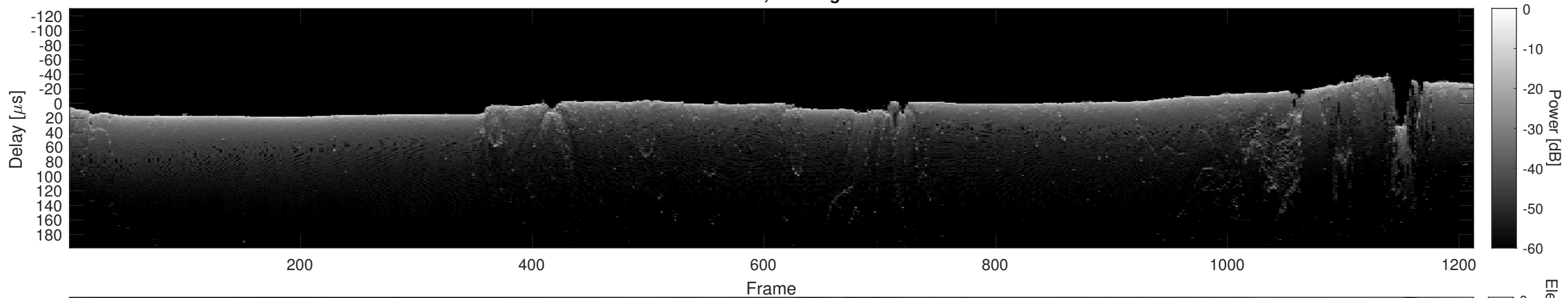
Orbit 11548, Cluttergram
