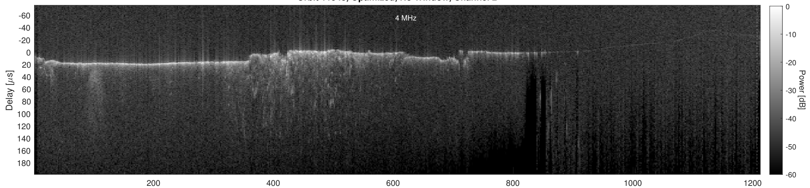
Orbit 11548, Cluttergram
