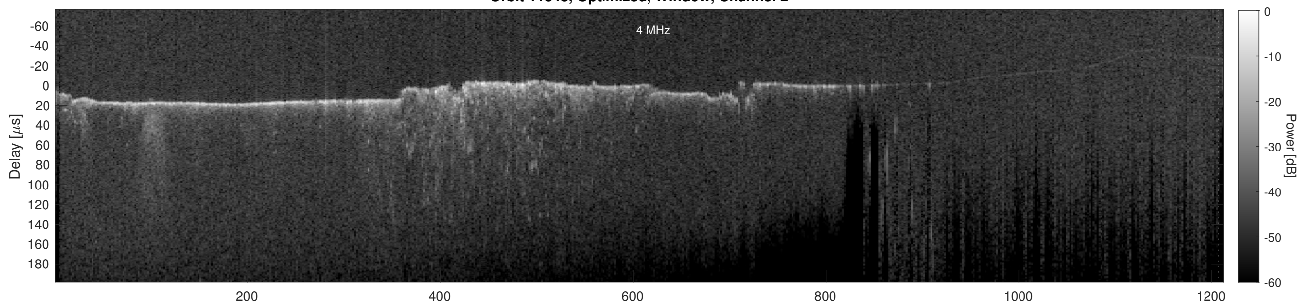
Orbit 11548, Cluttergram
