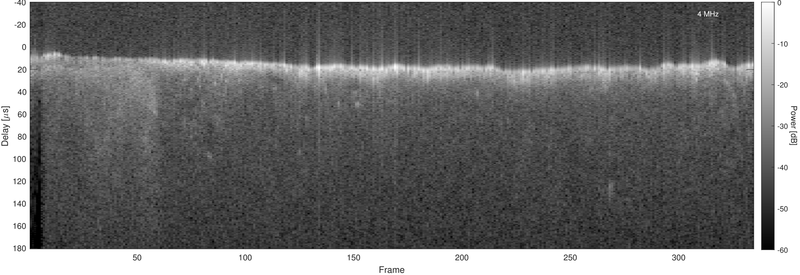
Orbit 11549, Chapman, No Window, Channel 2
