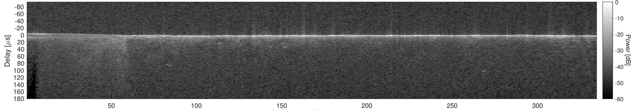
Orbit 11549, Cluttergram
