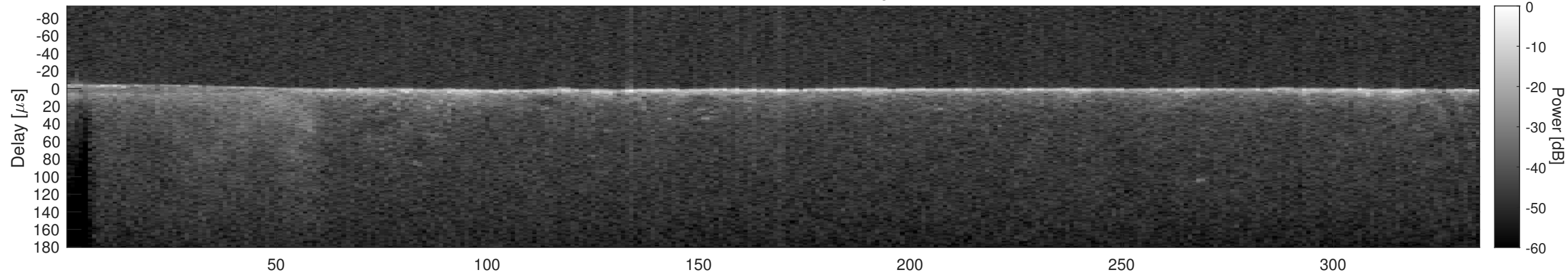
Orbit 11549, Cluttergram
