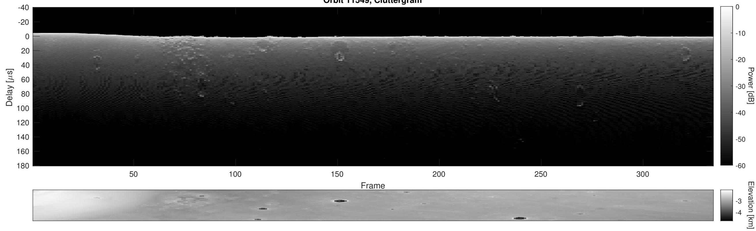
Orbit 11549, Cluttergram
