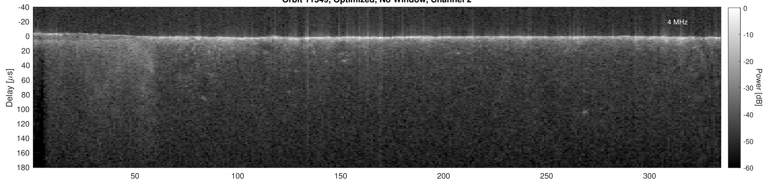
Orbit 11549, Cluttergram
