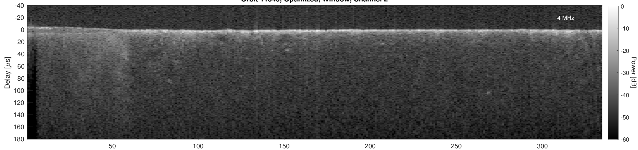
Orbit 11549, Cluttergram
