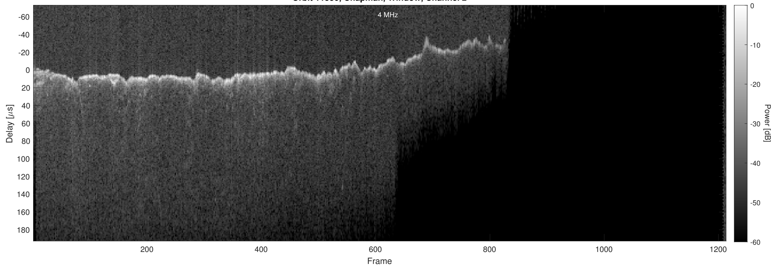
Orbit 11550, Chapman, Window, Channel 2
