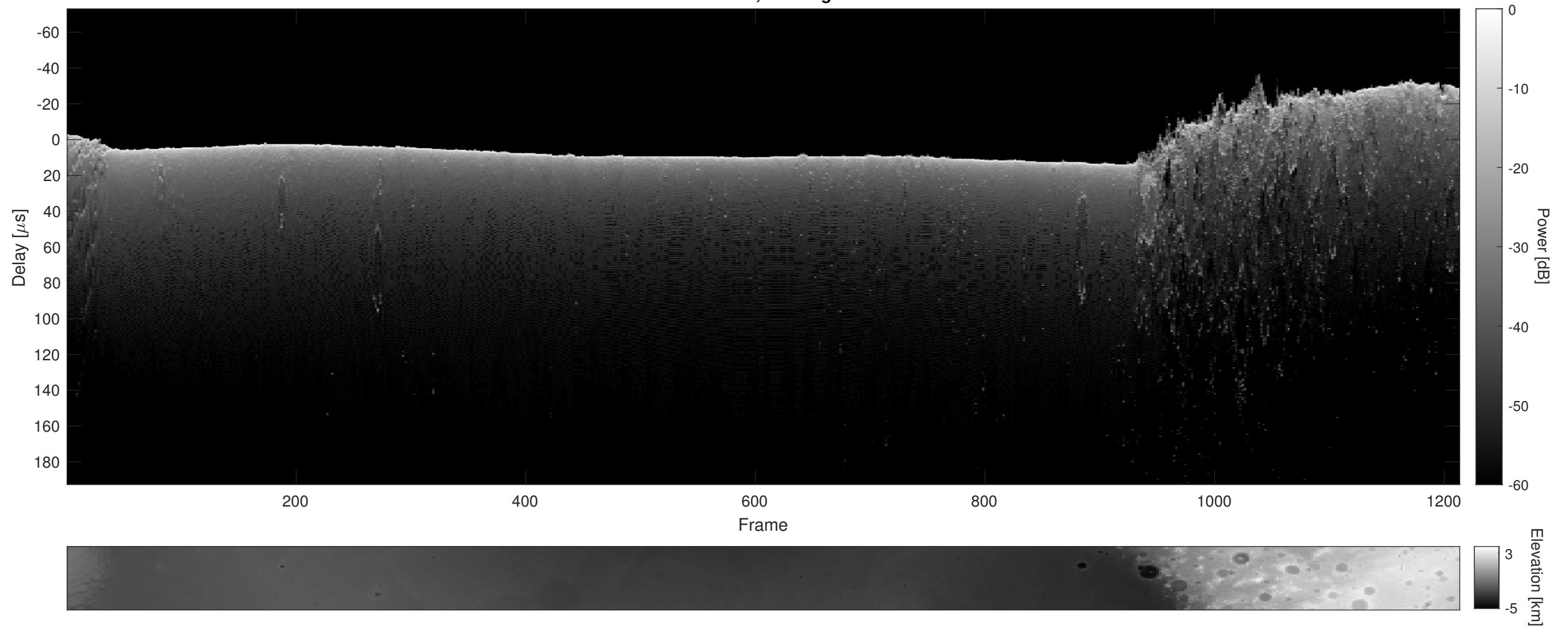
Orbit 11550, Cluttergram
