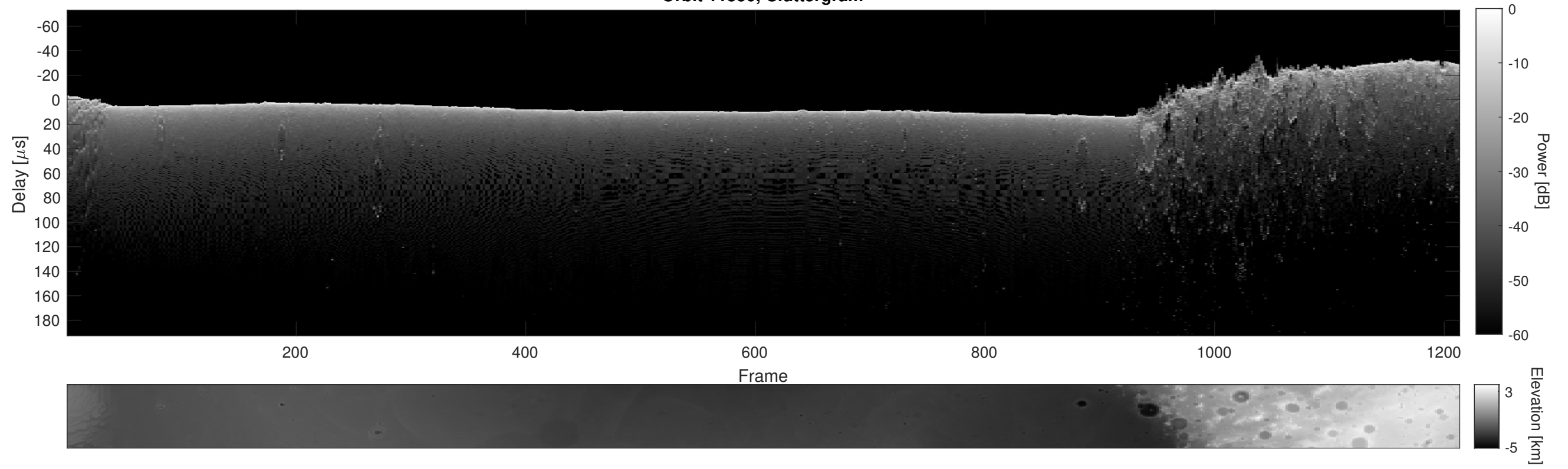
Orbit 11550, Cluttergram
