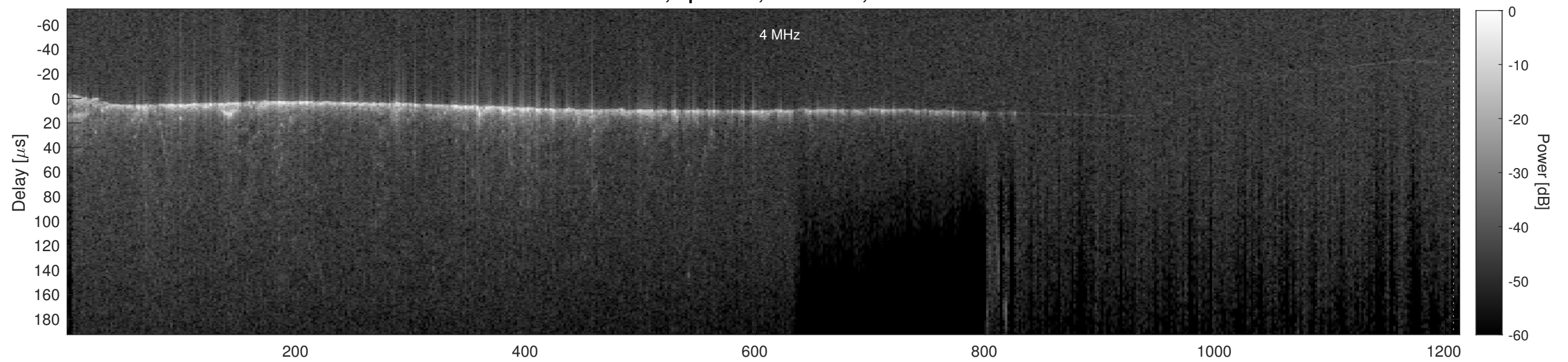
Orbit 11550, Cluttergram
