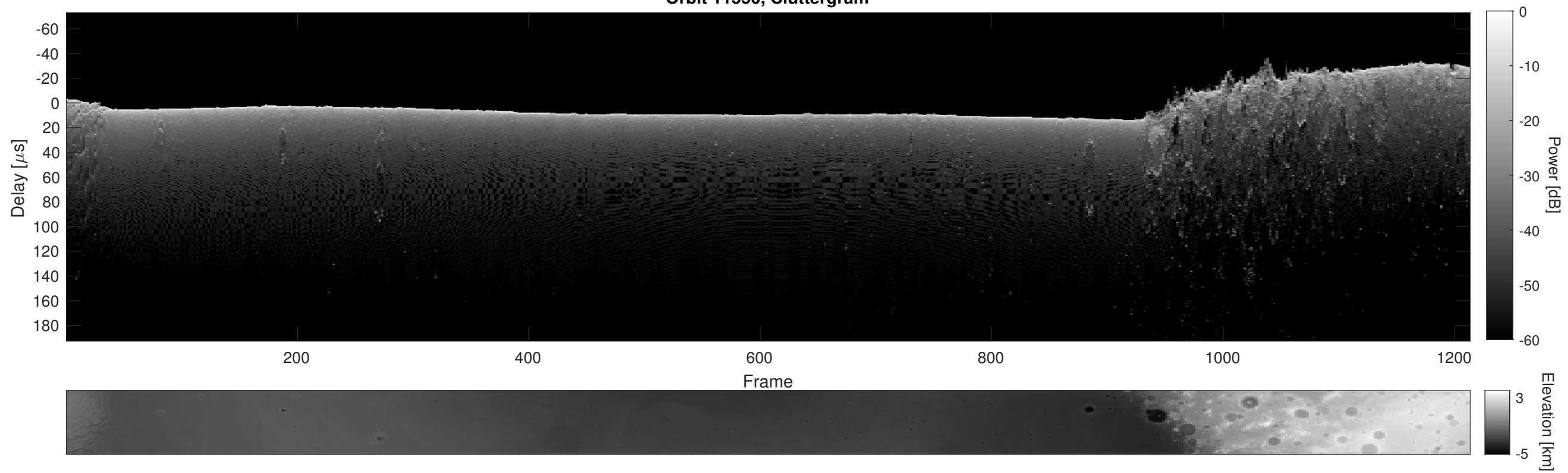
Orbit 11550, Cluttergram
