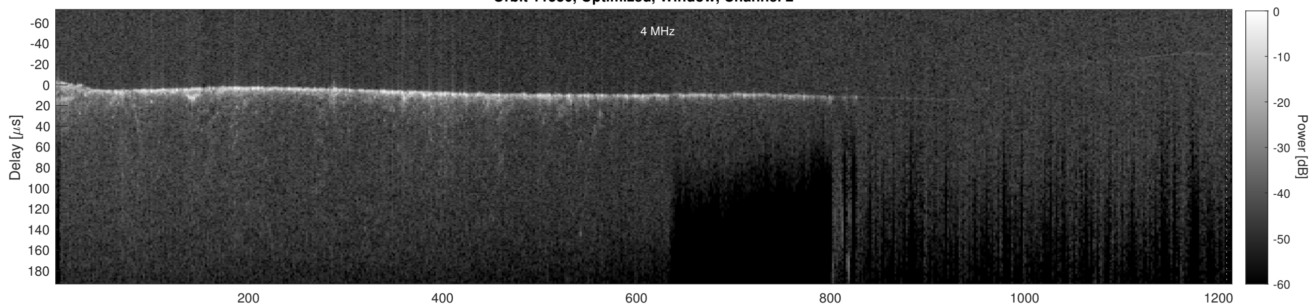
Orbit 11550, Cluttergram
