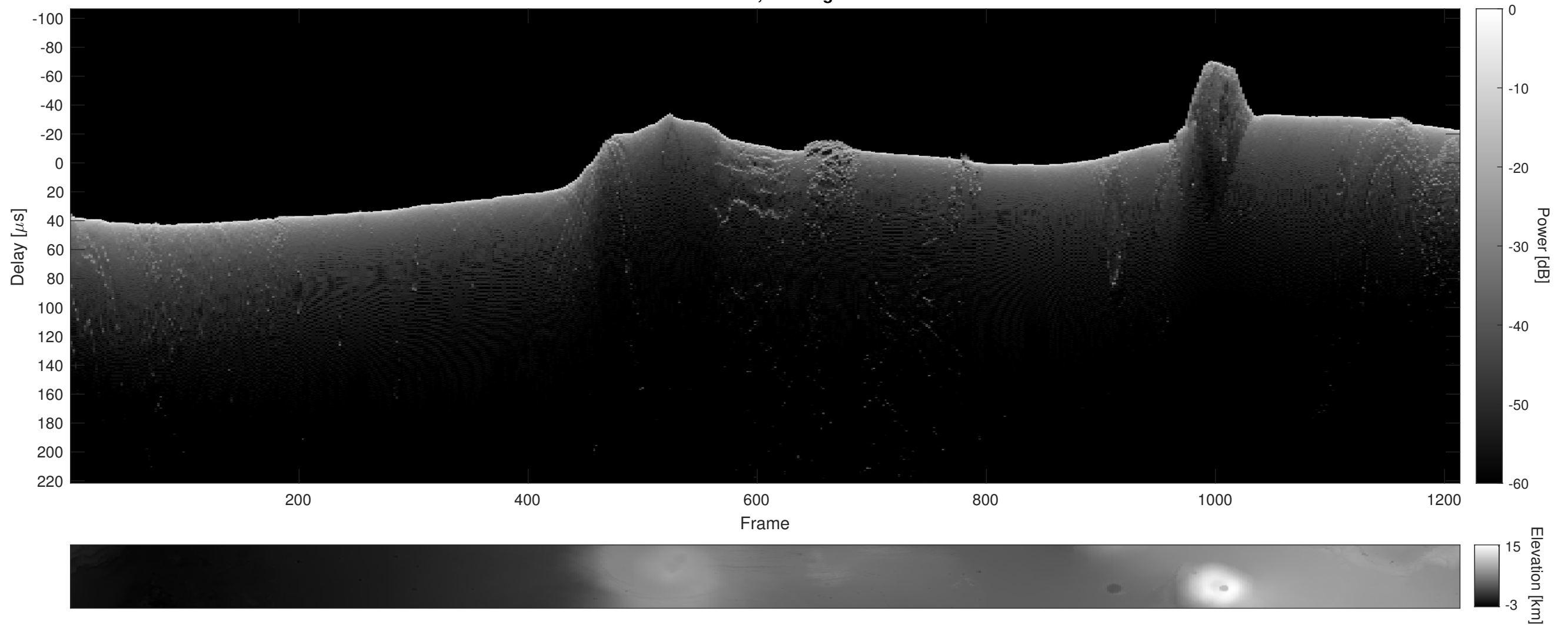
Orbit 11552, Cluttergram
