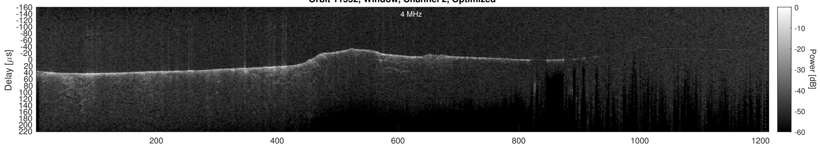
Orbit 11552, Cluttergram
