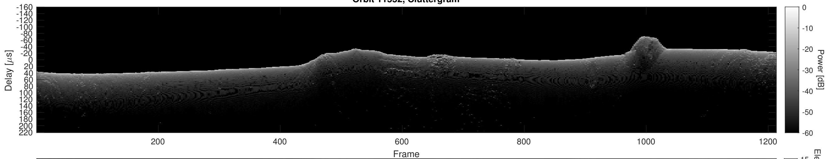
Orbit 11552, Cluttergram
