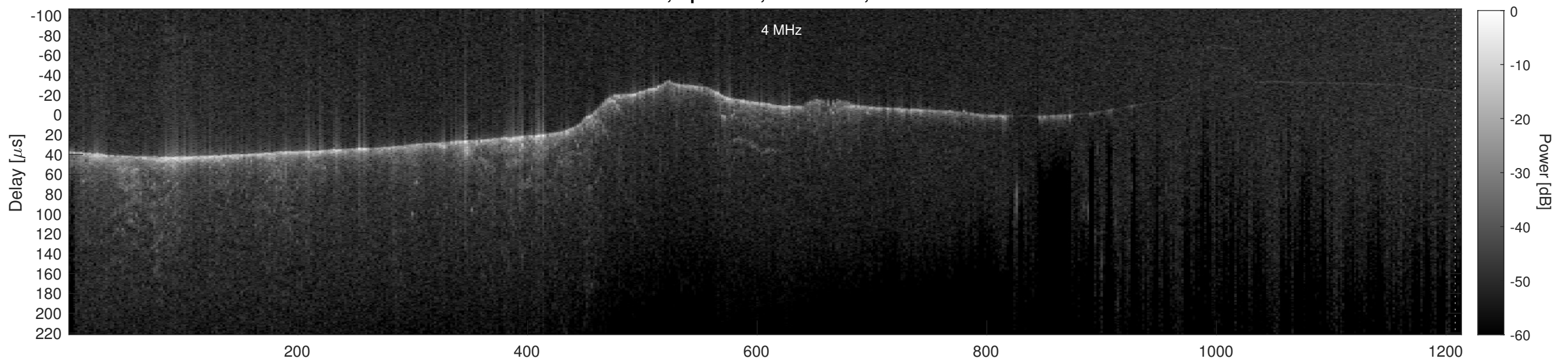
Orbit 11552, Cluttergram
