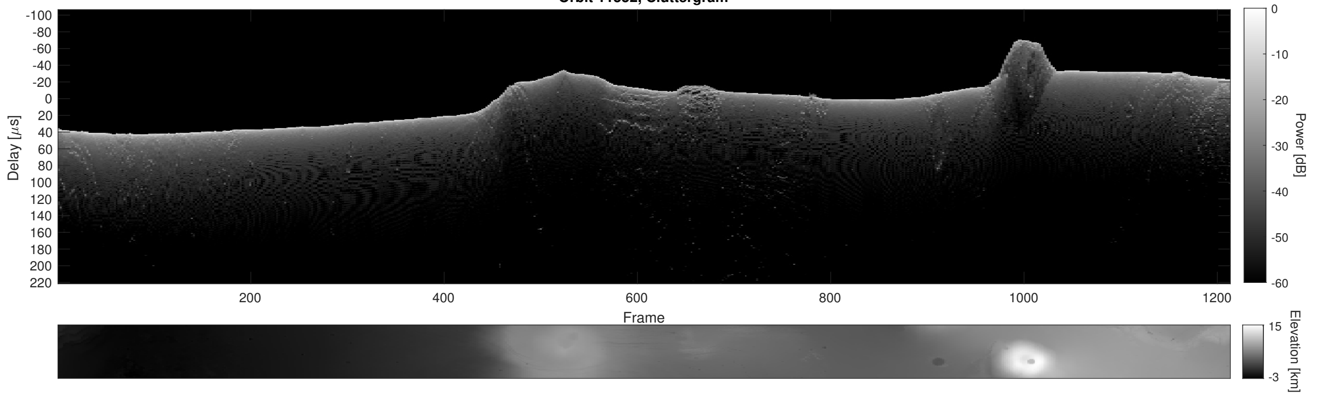
Orbit 11552, Cluttergram
