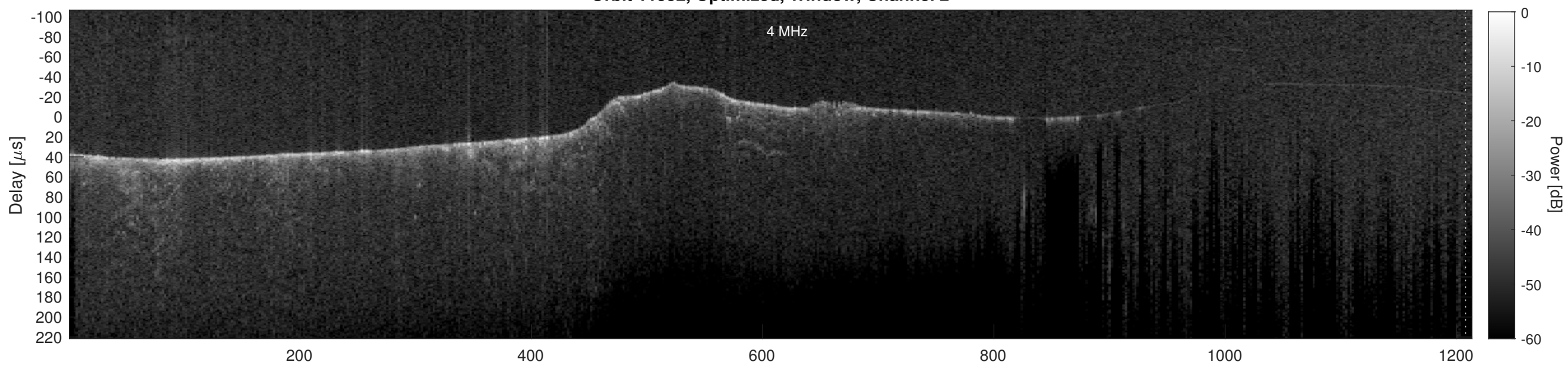
Orbit 11552, Cluttergram
