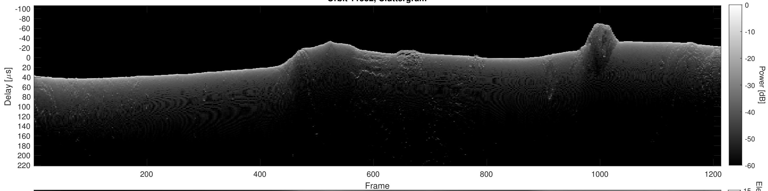
Orbit 11552, Cluttergram
