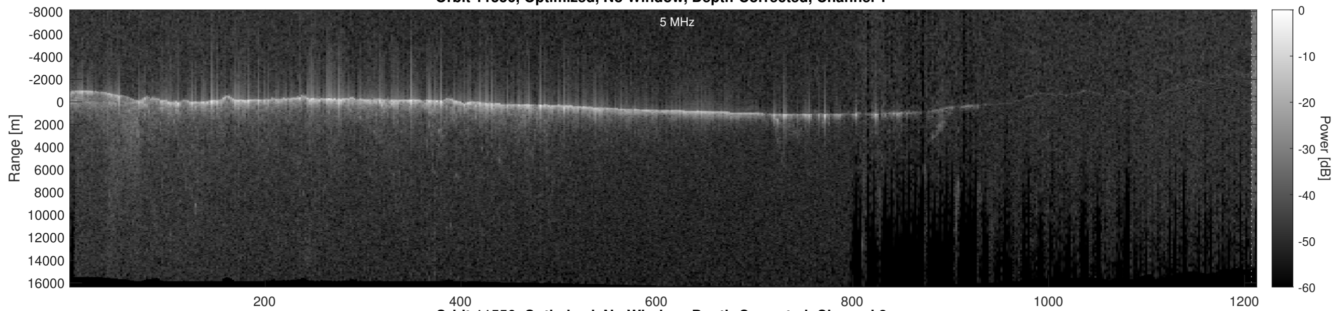
Orbit 11556, Optimized, No Window, Depth-Corrected, Channel 2
