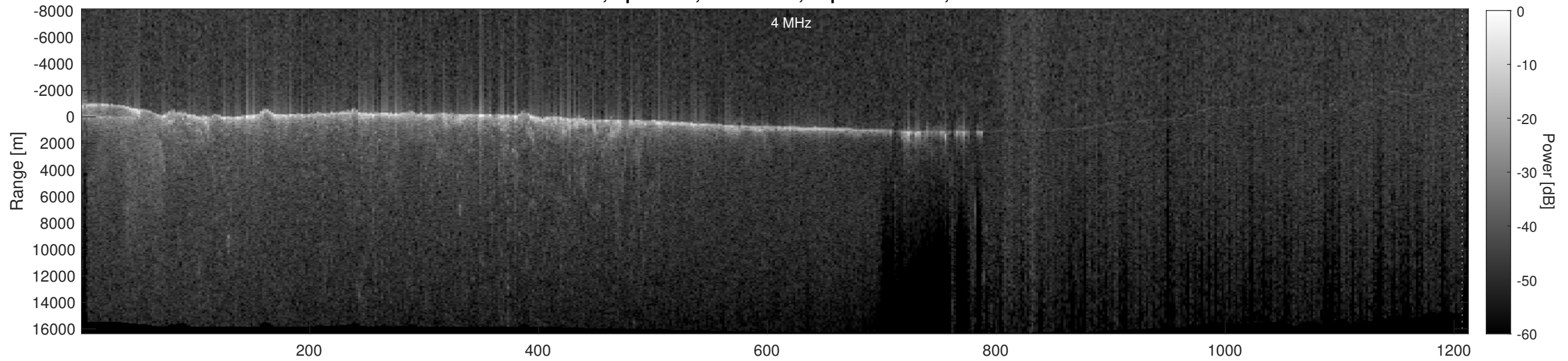
Orbit 11556, Depth-Corrected Cluttergram
