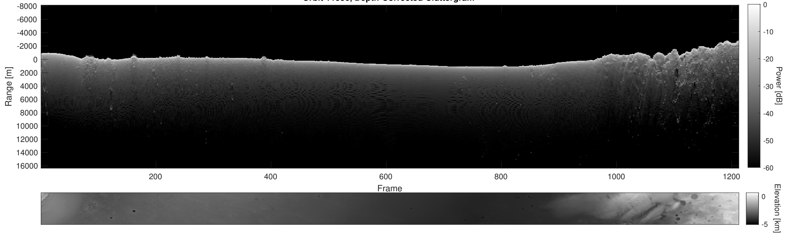
Orbit 11556, Depth-Corrected Cluttergram
